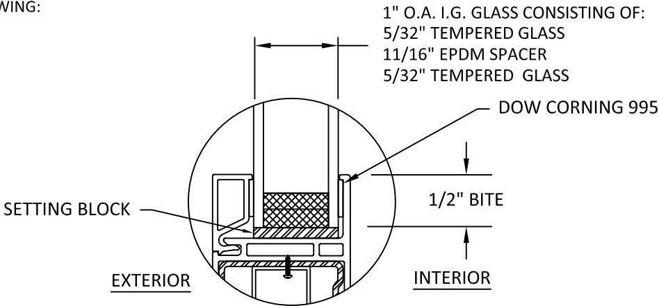
GLAZING DETAIL
