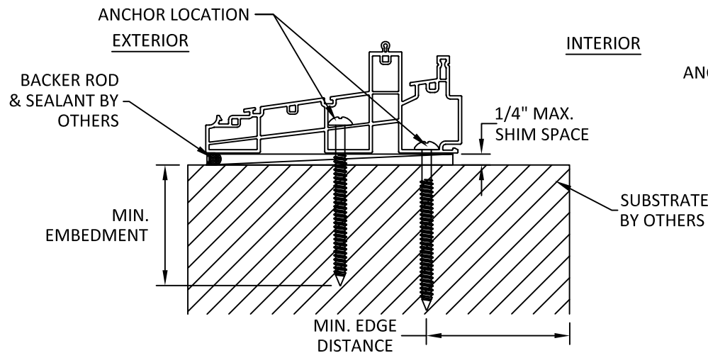
B 5 ANCHOR DETAIL THROUGH FRAME
