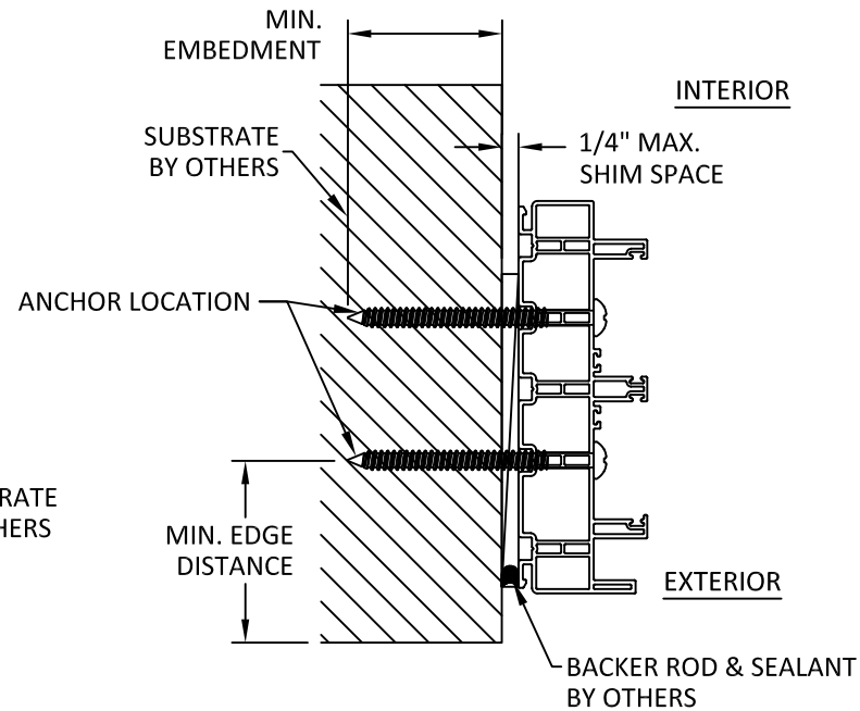
C 5 ANCHOR DETAIL THROUGH FRAME
