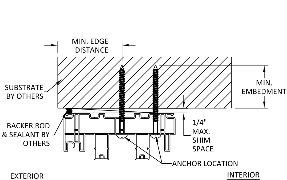
A 5 ANCHOR DETAIL THROUGH FRAME
